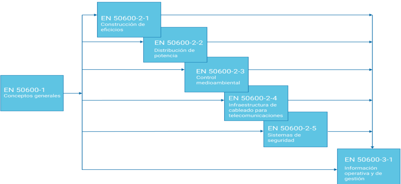
The structure of EN 50600
